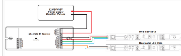
Wiring Diagram
