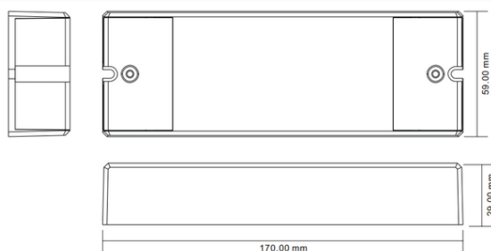
Product Dimension
