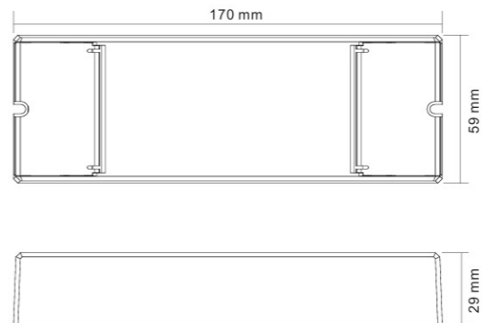
Product Dimension
