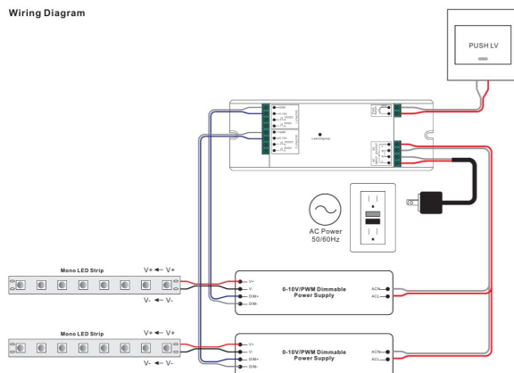
Wiring Diagram
