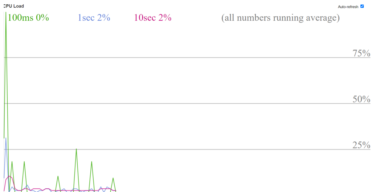
Figure 3-1.3: CPU Information
