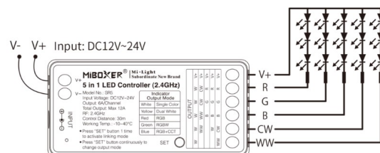
RGB+CCT mode
